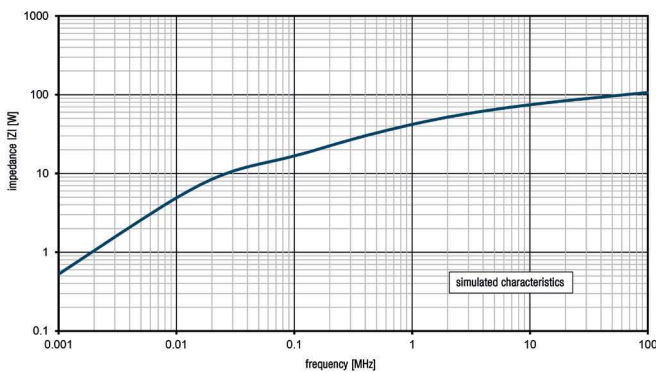
Fig. 1: Impedance |Z| [Ω] / frequency [MHz]
